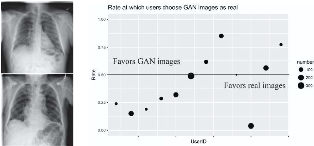
Figure 27.27 GAN generated images of lung X-rays. On the left, a pair consisting of a real X-ray and a GAN-generated X-ray. On the right, results of a test asking radiologists, given a pair of X-rays as seen on the left, to tell which is the real X-ray. On average, they chose correctly 61% of the time, somewhat better than chance. But they differed in their accuracy—the chart on the right shows the error rate for 12 different radiologists; one of them had an error rate near 0% and another had 80% errors. The size of each dot indicates the number of images each radiologist viewed. Figure courtesy of Alex Schwing, produced by a system described in Deshpande et al. (2019).
