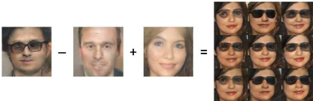
Figure 22.9 A demonstration of how a generative model has learned to use different directions in \mathbf{z} space to represent different aspects of faces. We can actually perform arithmetic in \mathbf{z} space. The images here are all generated from the learned model and show what happens when we decode different points in \mathbf{z} space. We start with the coordinates for the concept of “man with glasses,” subtract off the coordinates for “man,” add the coordinates for “woman,” and obtain the coordinates for “woman with glasses.” Images reproduced with permission from (Radford et al. , 2015).
